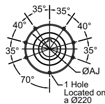
Gear Frame - Size 36
