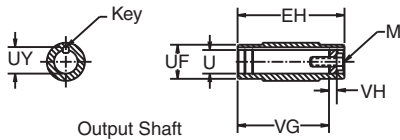
Output Shaft
