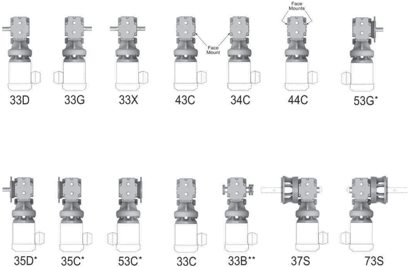
Examples Above are Top Views (with C-Face motor)
