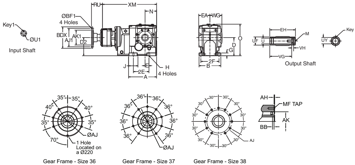
Gear Frame - Size 36
