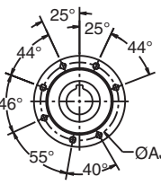
Gear Frame - Size 34
