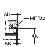
Input Shaft Frames 33, 34 and 35
