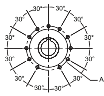
Gear Frame - Size 38
